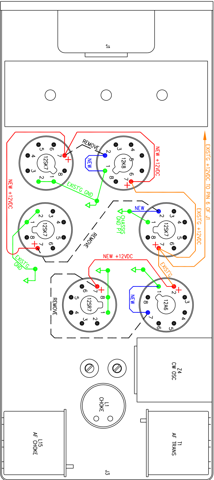
ARC-5 RECEIVER 28VDC TO 12VDC HEATER REWIRING
